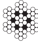
7 x 7
